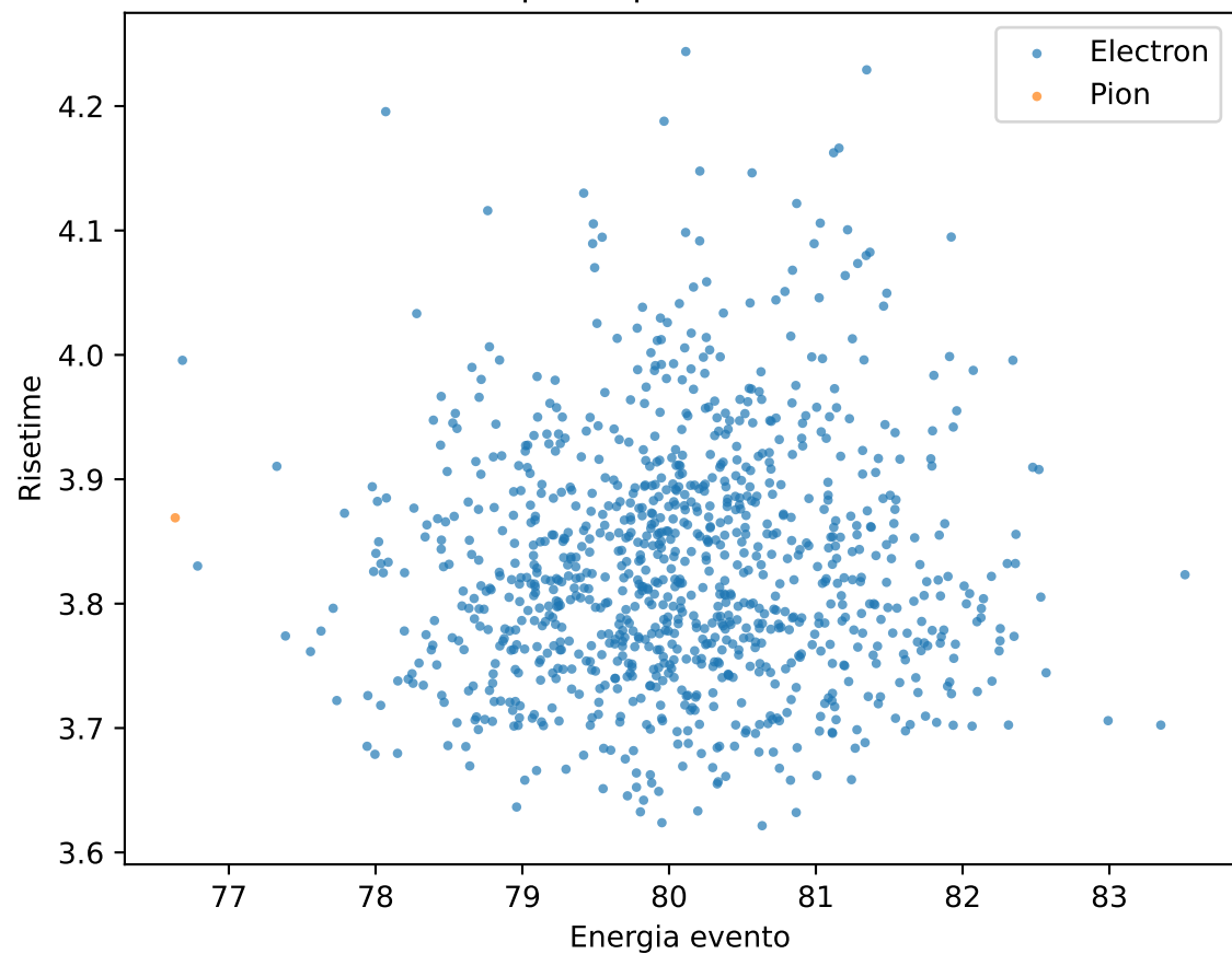
Scatter plot e/pi (cutted) 80.0GeV
