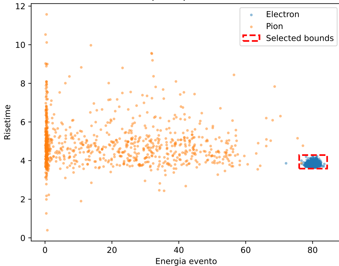
Scatter plot e/pi (all) 80.0GeV
